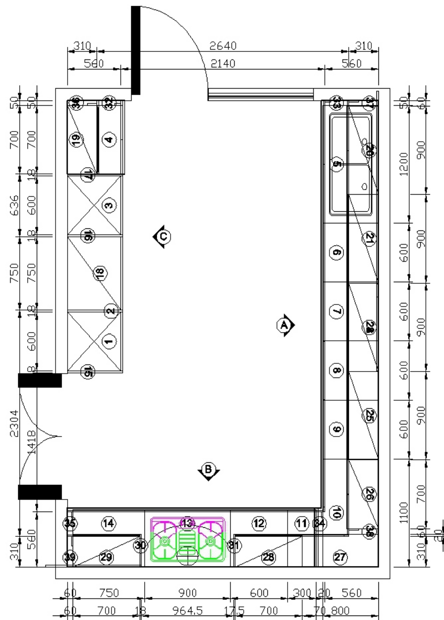
Plan drawing
